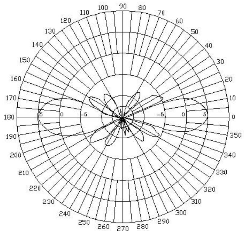
E-Plane Field Pattern
